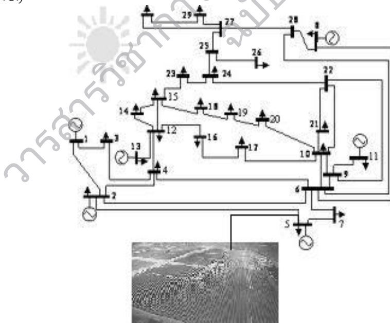
Figure.2: Location of solar farm in IEEE 30 bus tests system
