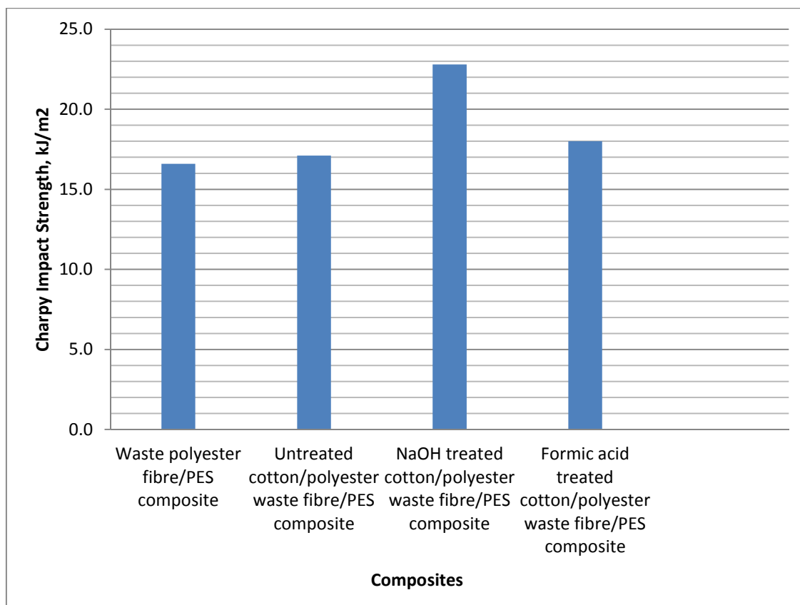
Figure 1. Charpy impact strength properties of the waste fibre polymer composites
