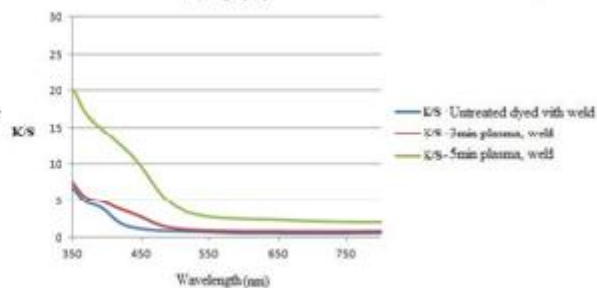
Figure 7: the Reflectance factor and relative color strength for the dyed samples with weld.
