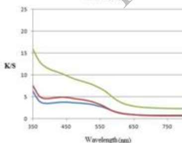
Figure 6- reflective spectra for dyed samples with madder.
