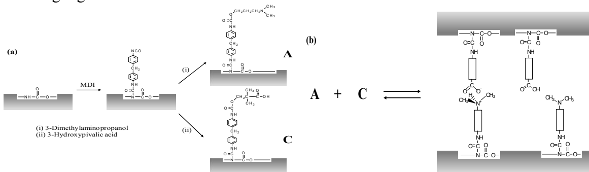
Figure 1: (a) PU grafting with dimethylamino group (A) or carboxyl group (C), and (b) ionic crosslinking equilibrium between A and C (the box designates MDI unit)
