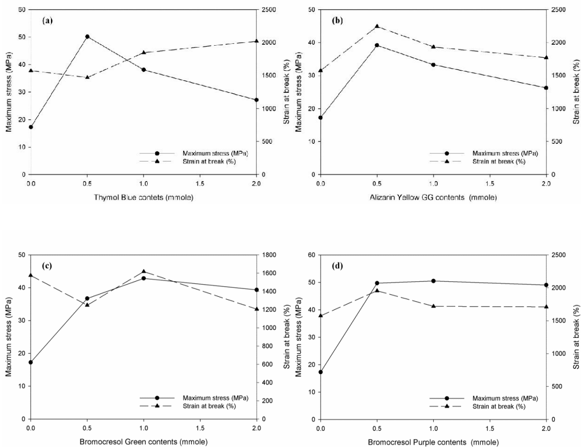
Figure 2: Maximum stress and strain at break of (a) Thymol Blue, (b) Alizarin Yellow GG, (c) Bromocresol Green, and (d) Bromocresol Purple series.
