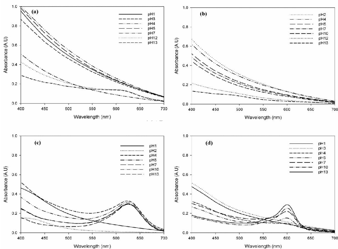
Figure 1: Spectral changes of PU solution grafted with (a) Thymol Blue, (b) Alizarin Yellow GG, (c) Bromocresol Green, and (d) Bromocresol Purple at different pH values.
