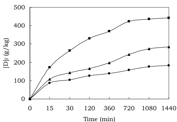
Figure 2: Plots of dye uptake with respect to time for (■) pre-oxidised wool, (▲) wool and (●) silk dyed with Punica granatum
